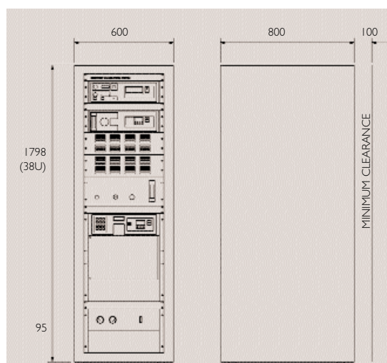
System shown: DCS80 Dimensions mm
