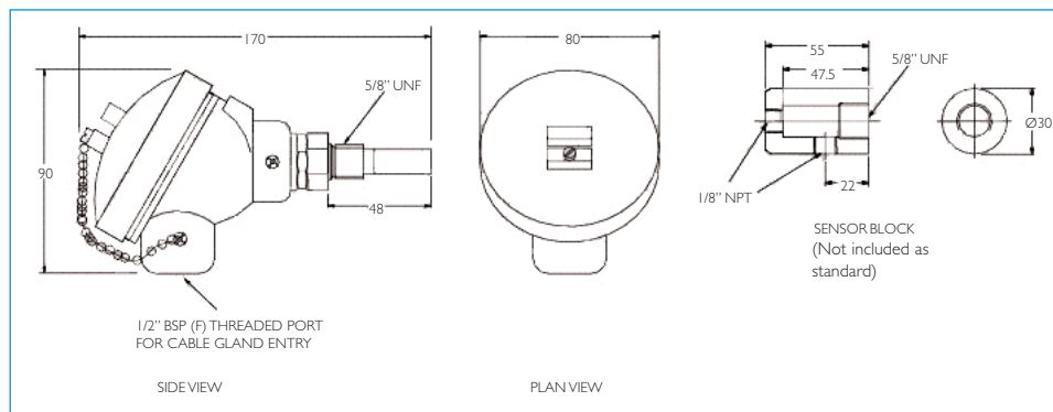
Dimensions mm
